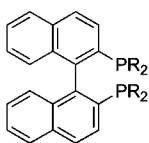
Binap, R = Ph 7
